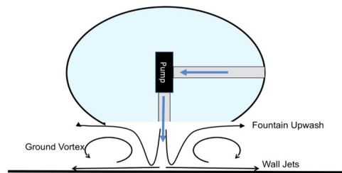
Fig. 6: Use of jet induced hydrodynamics for fluid bed formation and height control
