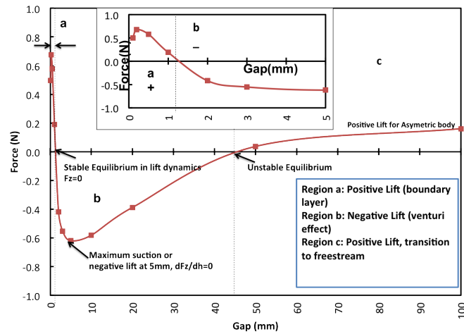
Fig. 5: Shows the three regimes: (a) h/c \leq 0 : 01 (b) 0 : 01 \leq h/c \leq 0 : 3 (c) 0 : 01 \leq h/c \leq 0 : 3 and how F_g acts in each for EVIE moving at 0.5m/sec
