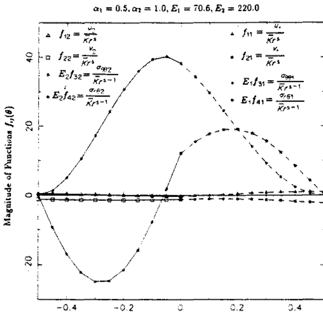
Fig. 2. Angular dependence of the eigenfunctions for \text{Si}_3\text{N}_4/\text{Al} .
